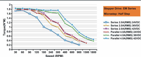
Stepper Motor: 57HS13
